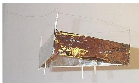
Lifter 1 – JL Naudin Experimental Model
